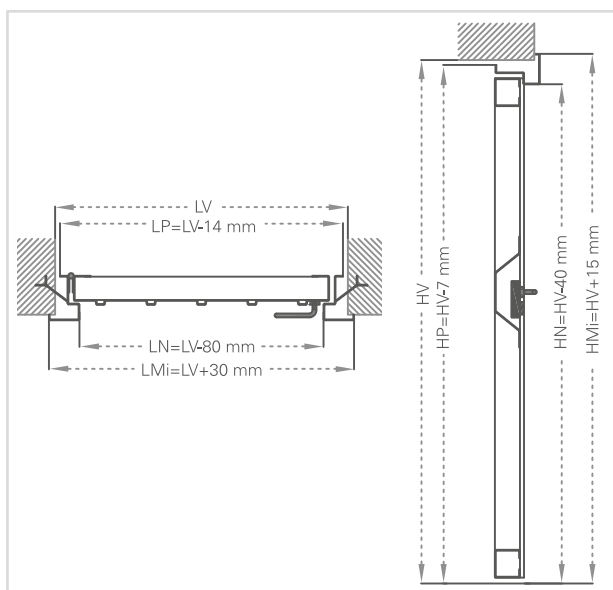
MOD. LIGHT - SPINGERE
